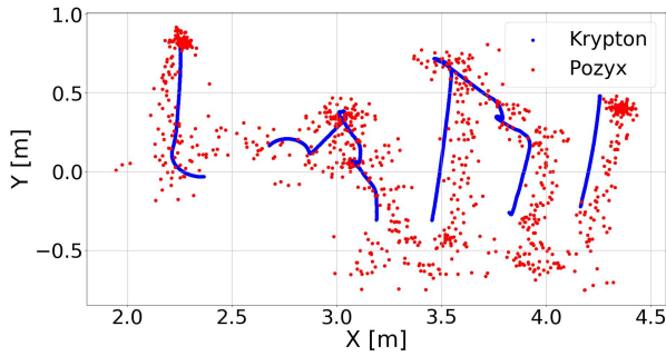
Figure 6. Pozyx positioning results (red) alongside Krypton CMM measurements (blue).
